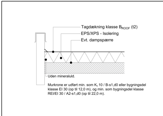
Figur 6.1 - Murkrone uden behov for mineraluld
